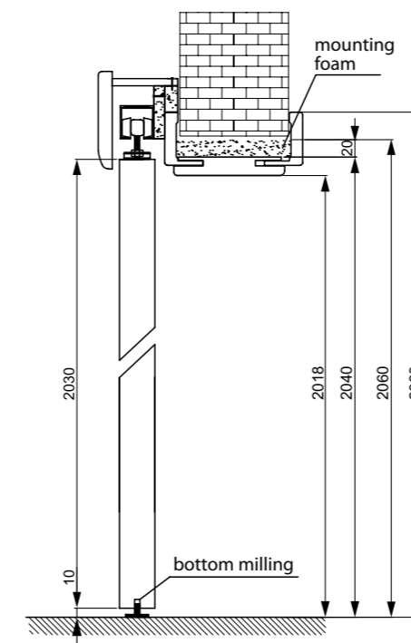
TUNNEL MOUNTING
