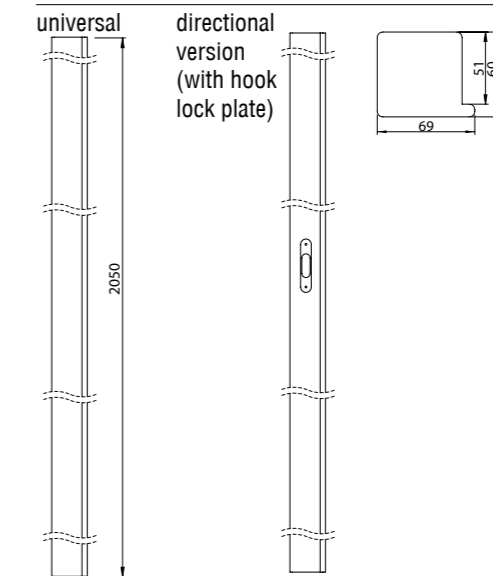
FENDER BEAM
