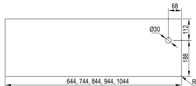
Protective central panel with drilling for economy lock
