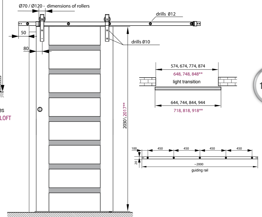
double system
