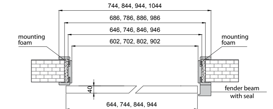
FENDER BEAM
